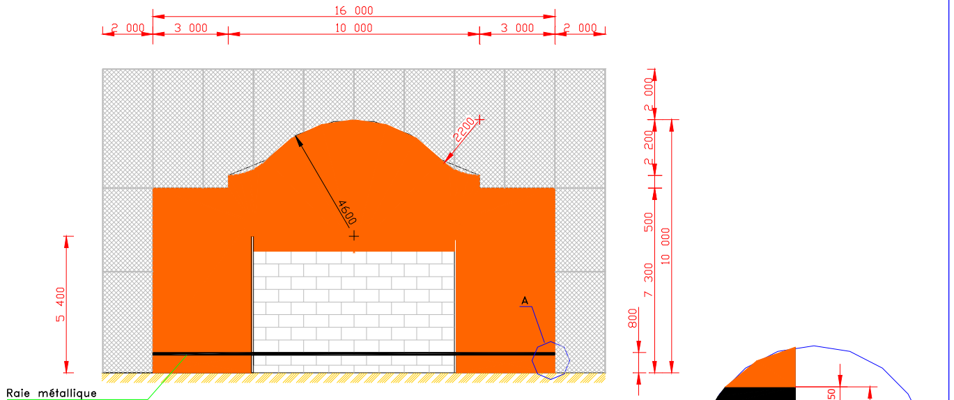
ELEVATION – FRONTON
